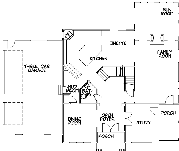
FIRST FLOOR PLAN LIVING AREA 1823 SF
