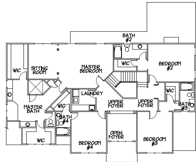
SECOND FLOOR PLAN LIVING AREA 2070 SF ( DNI OPEN AREAS )
