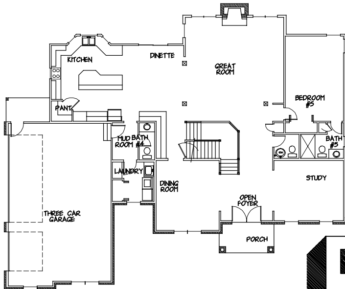
FIRST FLOOR PLAN LIVING AREA 2173 SF
