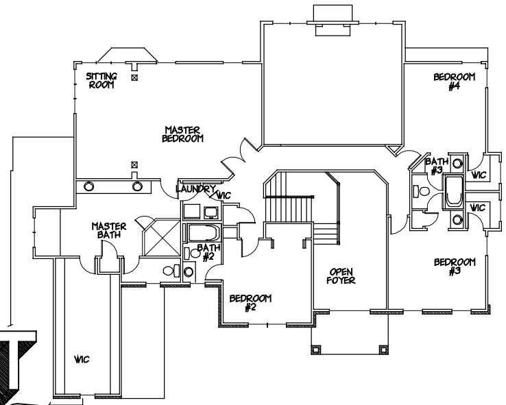
SECOND FLOOR PLAN LIVING AREA 2057 SF ( DNE OPEN AREAS )
