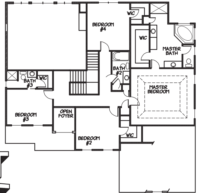
SECOND FLOOR PLAN LIVING AREA 1538 SF < DNI OPEN AREAS >
