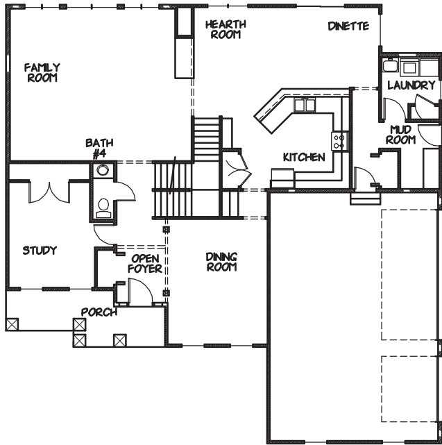
FIRST FLOOR PLAN LIVING AREA 1713 SF
